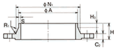
WELDING NECK
